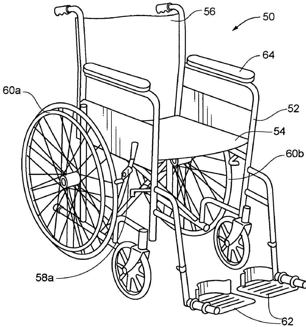
Fig. 1 Prior Art
